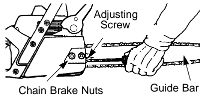
Chain Brake Nuts Adjusting Screw Guide Bar
